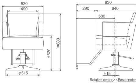
*Dimensions below show combination with chair base, SP-YE.
